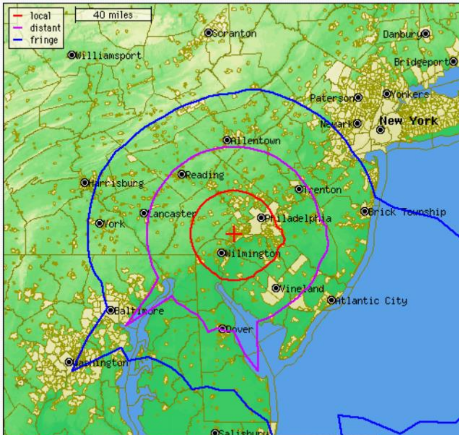
Daytime Coverage Pattern for WJFP-AM
