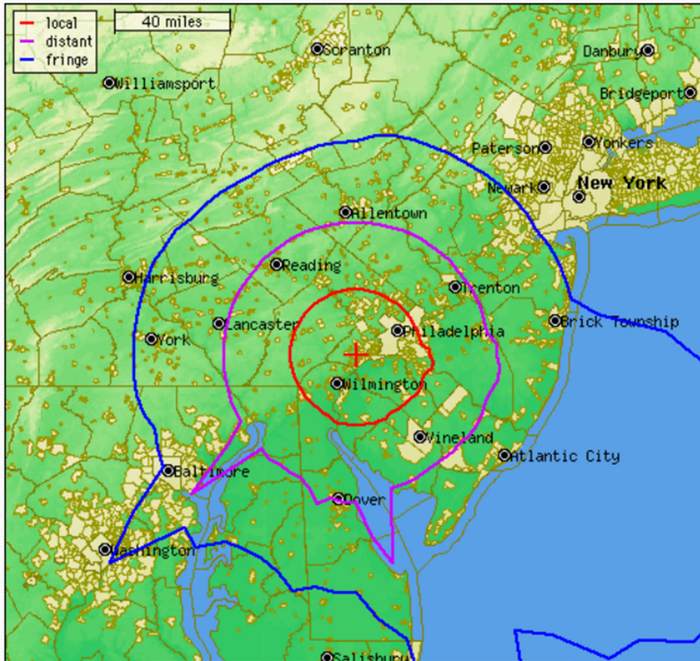
Daytime Coverage Pattern for WJFP-AM
